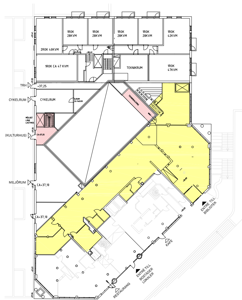
PLAN 0 ALT 2
