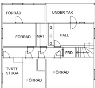
BOTTENPLAN
