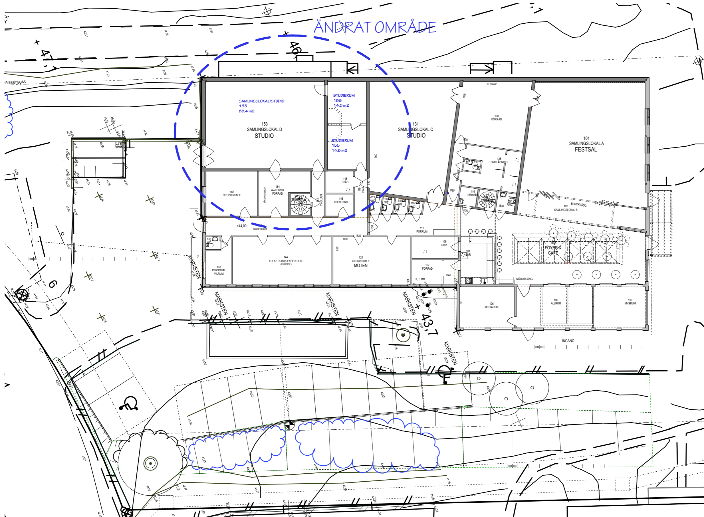
SITUATIONSPLAN
