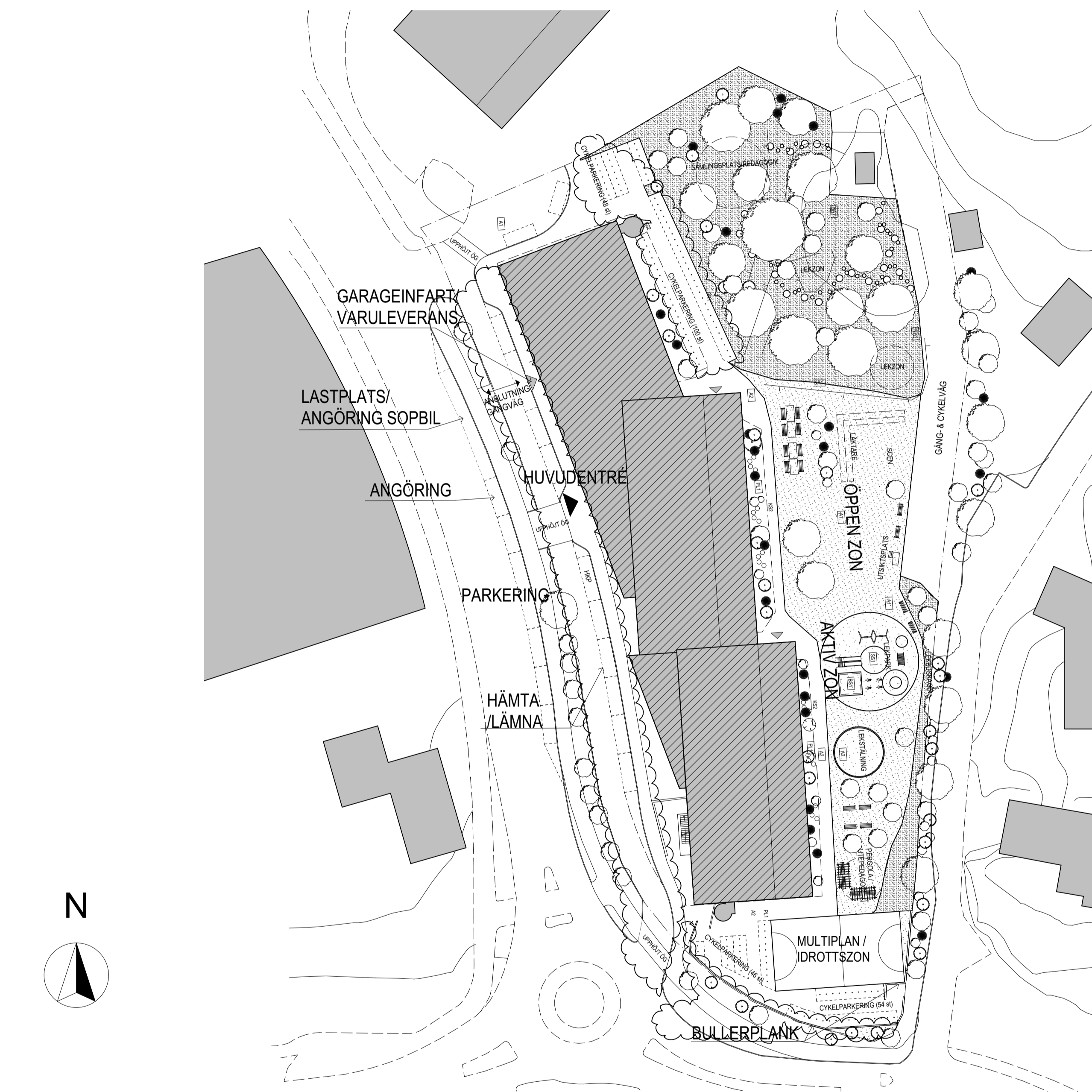
SITUATIONSPLAN / MARKPLAN
