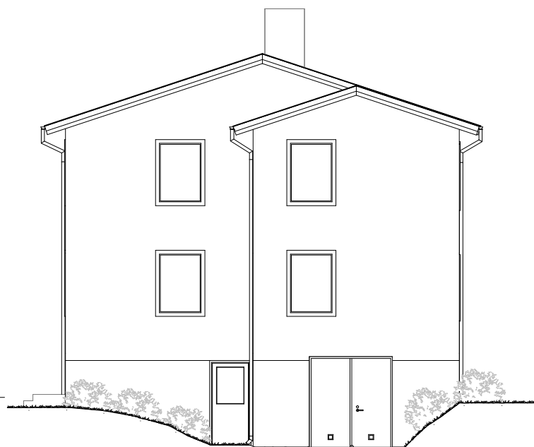
BEF. SITUATION FASAD MOT VÄSTER
