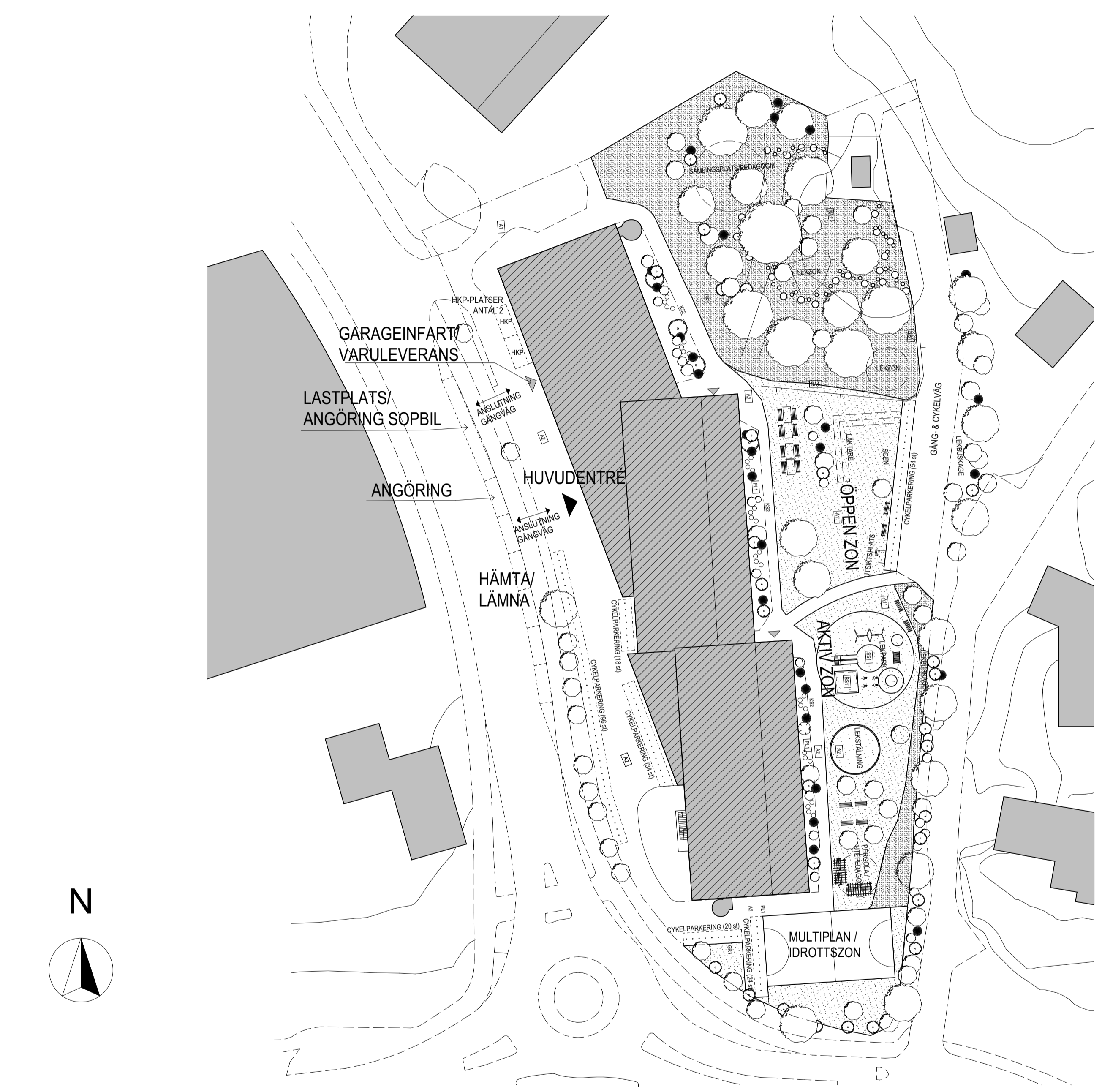
SITUATIONSPLAN / MARKPLAN
