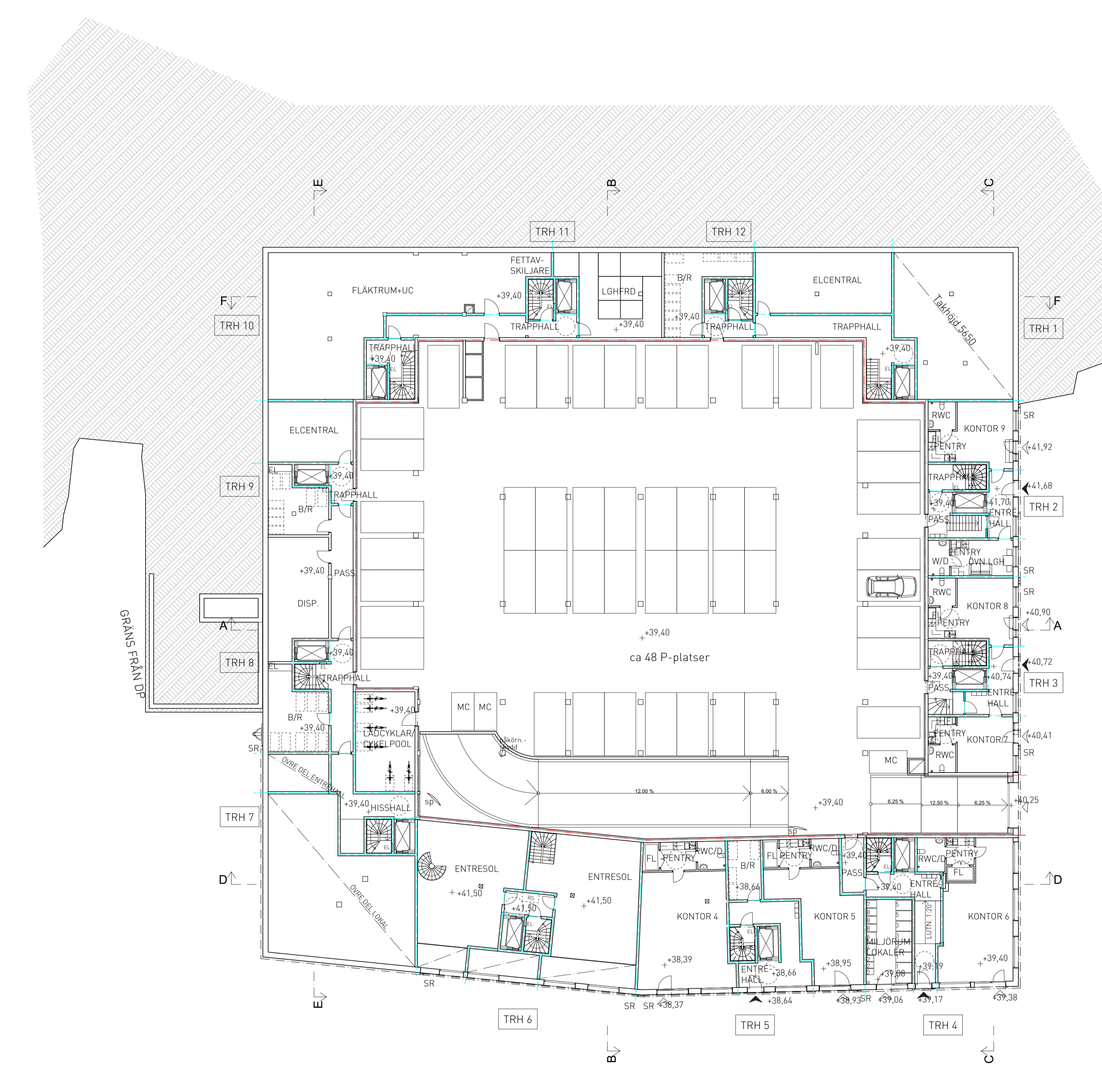
PLAN 11 1:200
