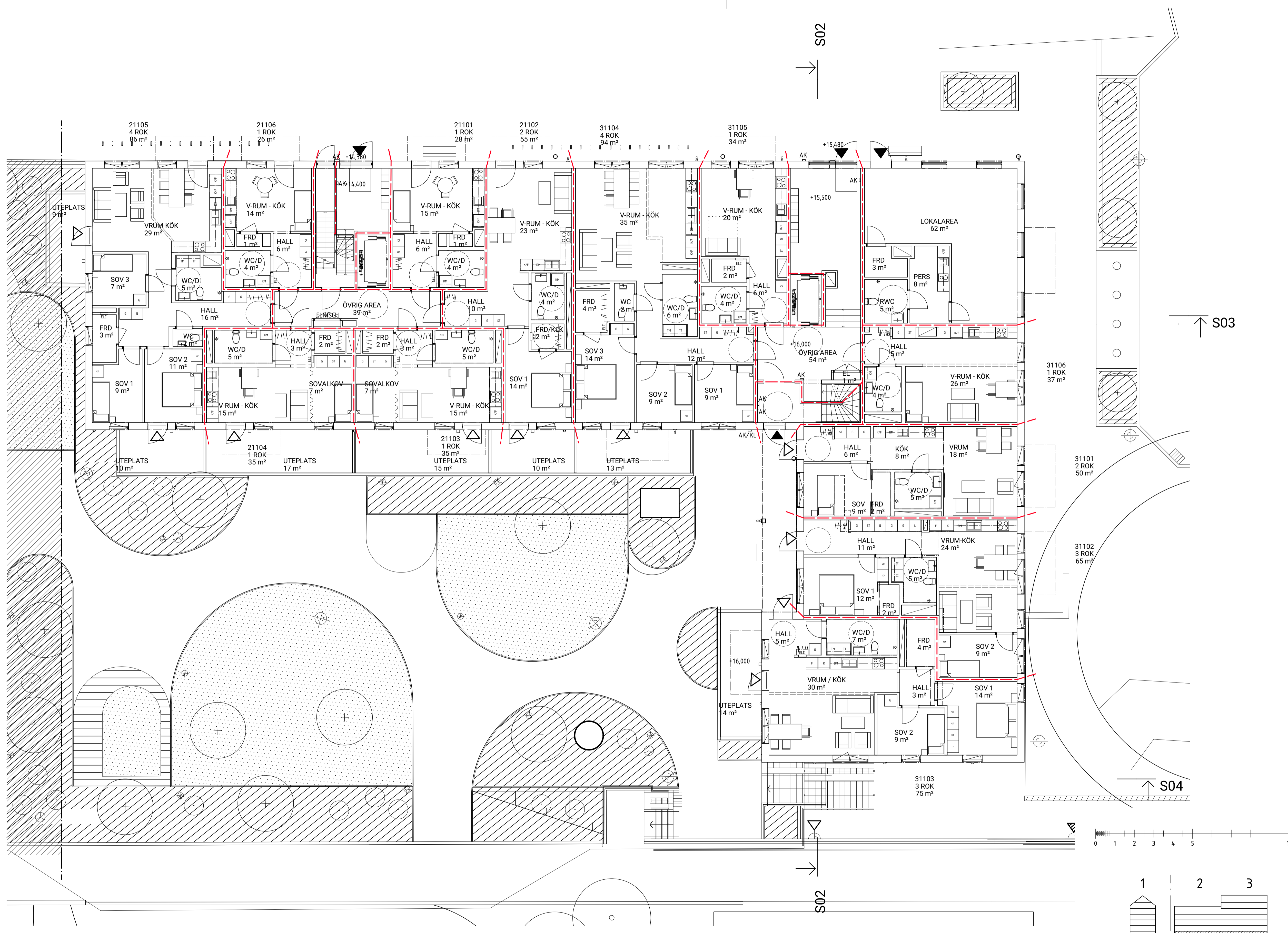
PLAN 11 (GÅRDSPLAN) 1:100
