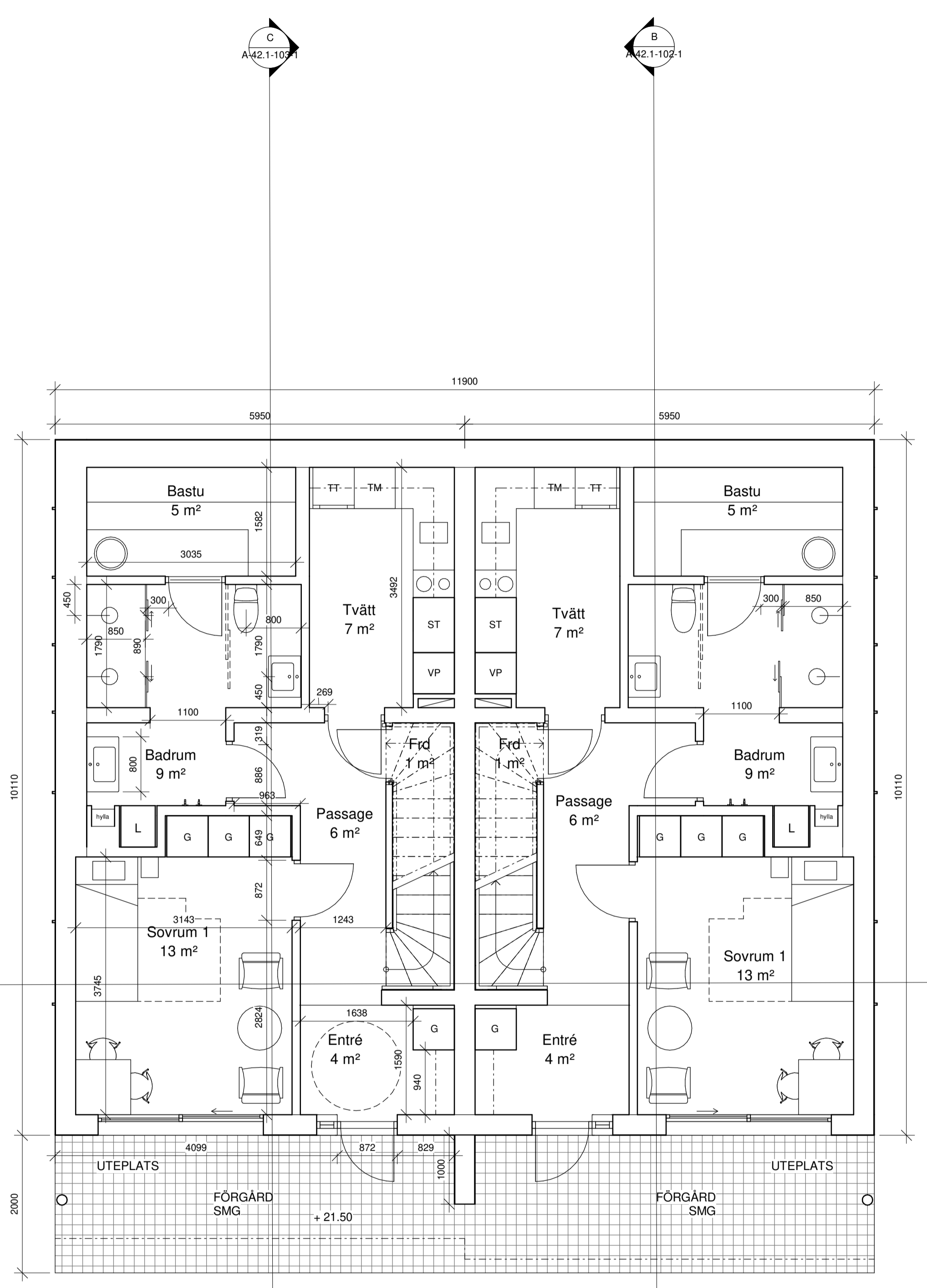
PLAN 0
